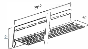
SV-11,5 Lower ventilation trim
