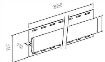
SV(P/PU)-18 Joint trim
