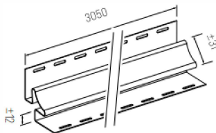
SV(P/PU)-13 Inside corner
